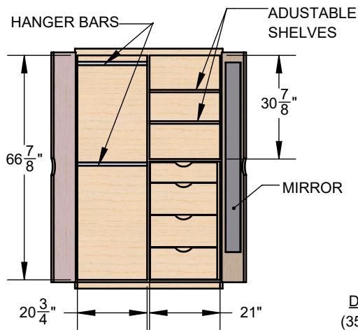
WARDROBE DETAIL
